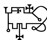
PHOENIX
